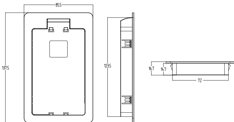
面板托架开孔尺寸: 123.5mm * 72mm
